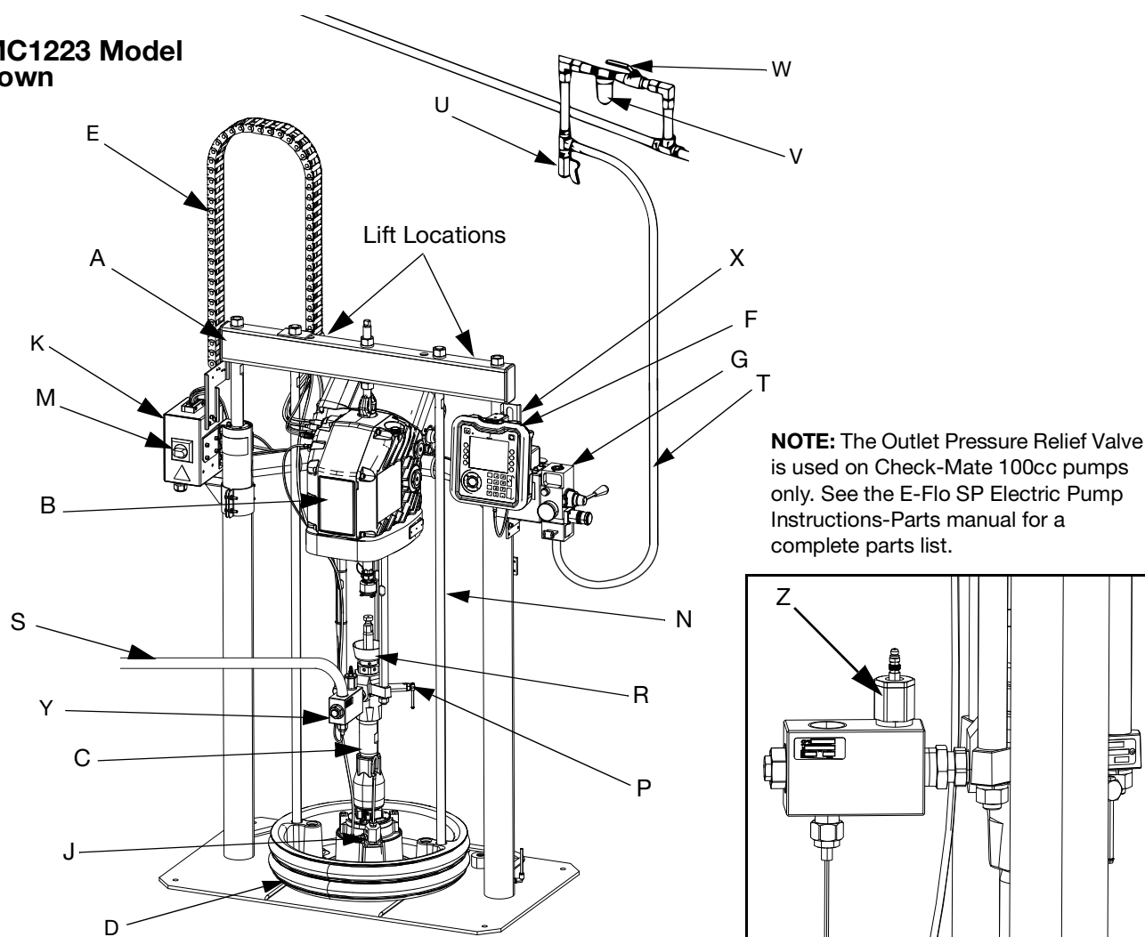
FIG. 1: Typical Installation
