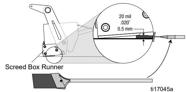
Screed Box
